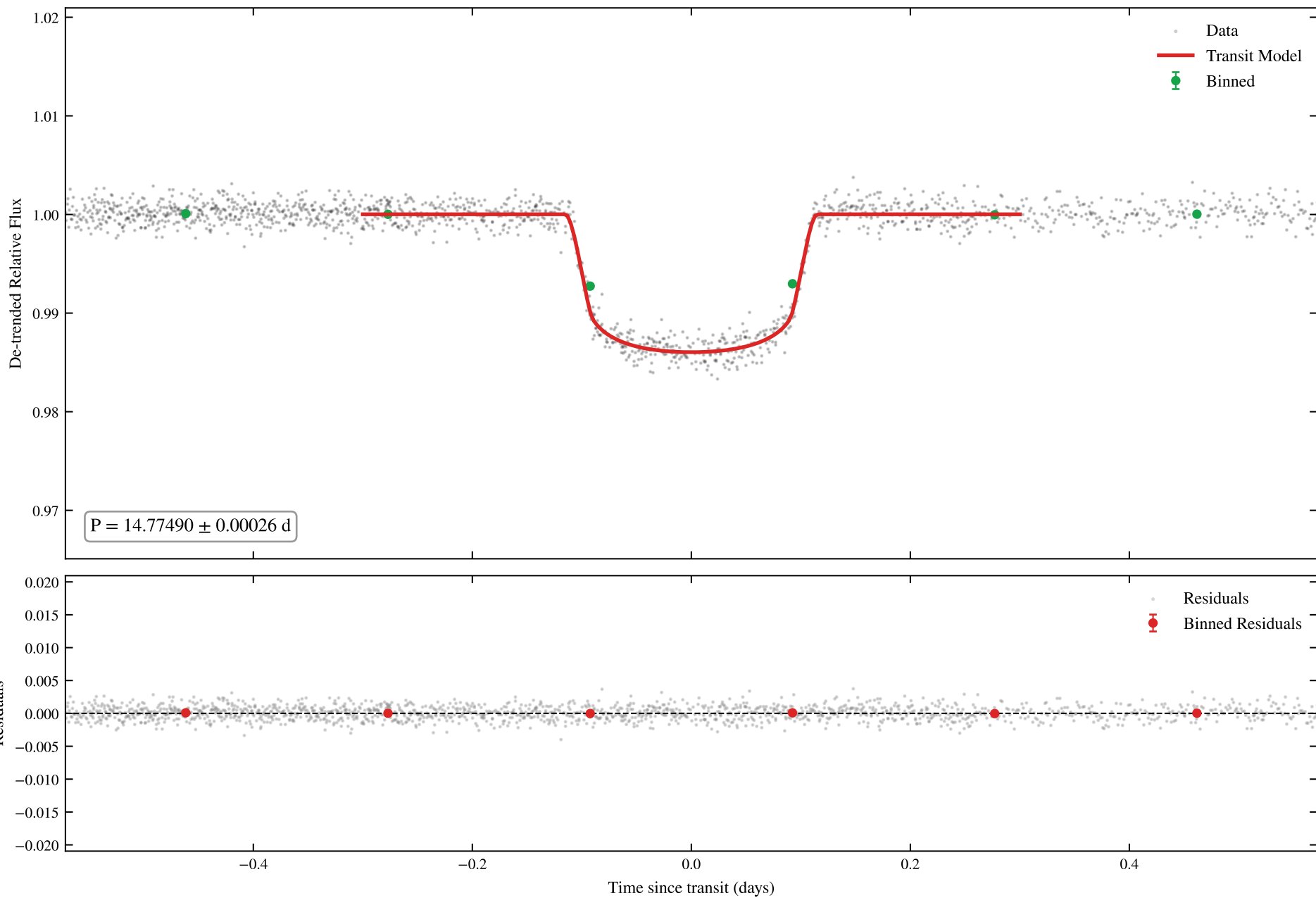
TIC 207081058 | Sectors: 105, 106 | Phased MCMC Fit - Planet 1
