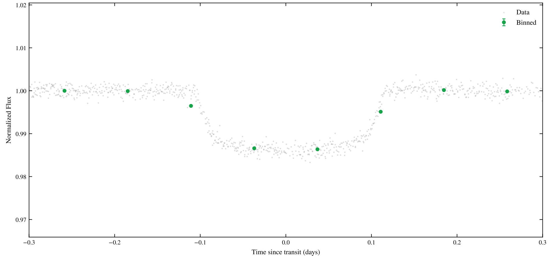
TIC 207081058 | Sectors: 105, 106 | Phase-Folded Transit (P = 14.77485 d)
