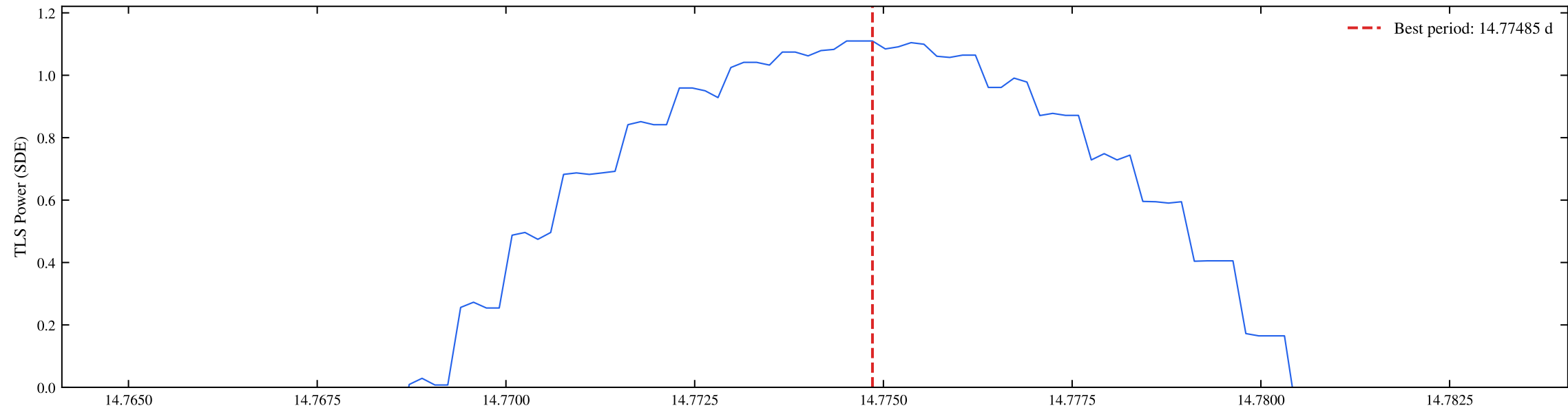
TIC 207081058 | Sectors: 105, 106 | TLS Periodogram (Planet 2 Search) (SDE = 4.82)
