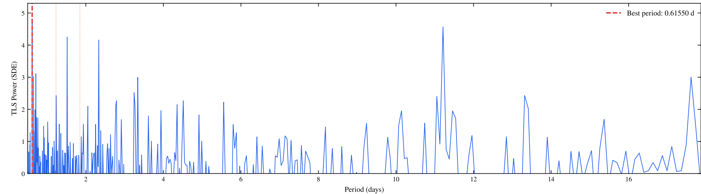
TIC 207081058 | Sectors: 105, 106 | TLS Periodogram (Planet 2 Search) (SDE = 4.82)
