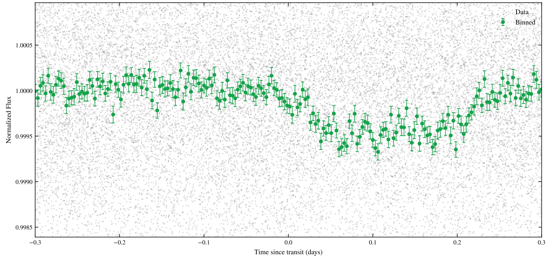
TIC 207081058 | Sectors: 105, 106 | Phase-Folded Transit (P = 0.61530 d)
