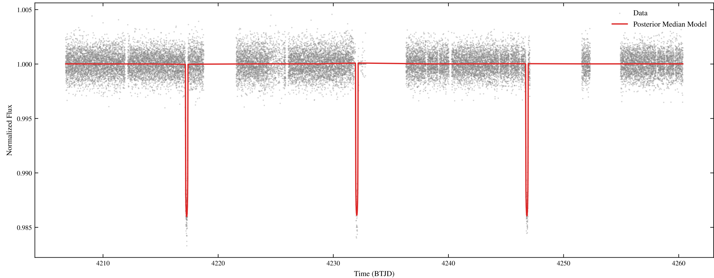
TIC 207081058 | Sectors: 105, 106 | MCMC Posterior Predictive Check
