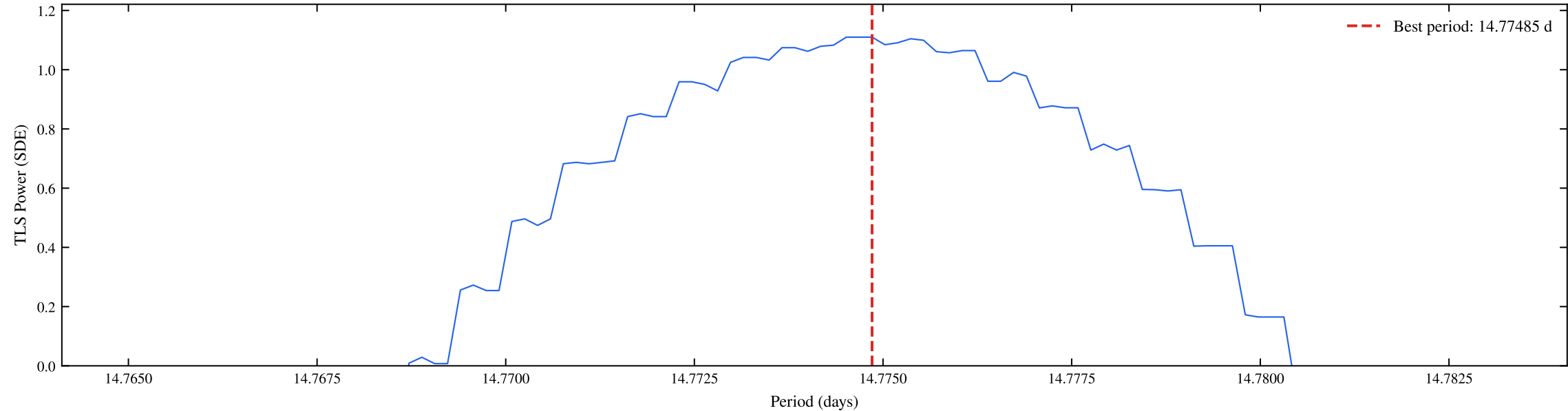
TIC 207081058 | Sectors: 105, 106 | TLS Fine Periodogram (SDE = 1.11)
