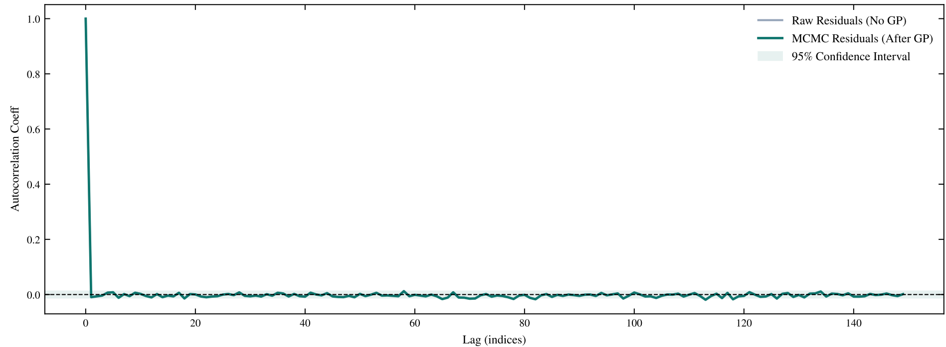
TIC 207081058 | Sectors: 105, 106 | GP Residuals Autocorrelation Function (ACF)
