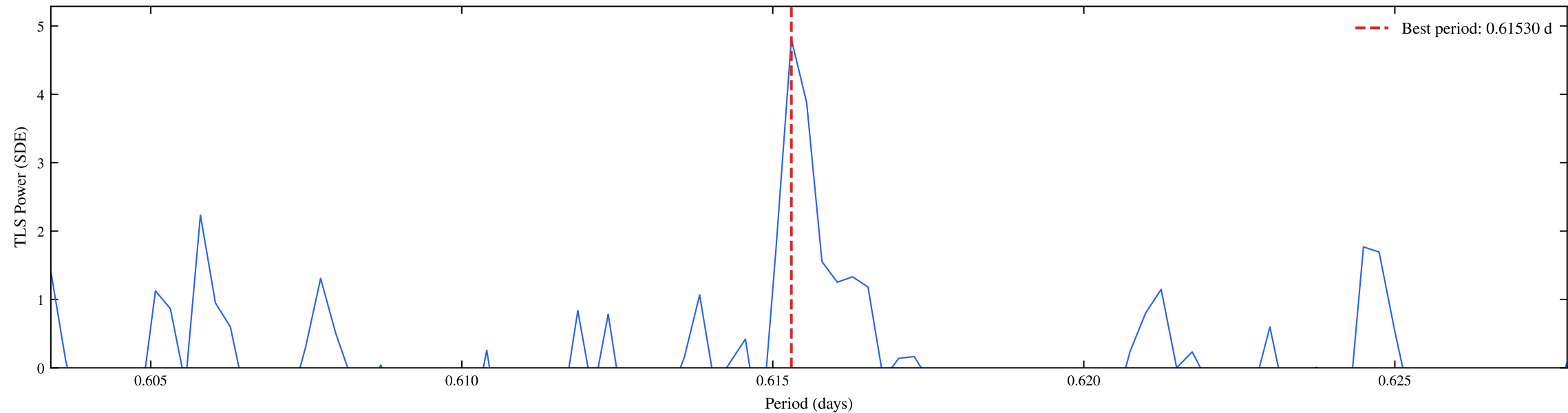
TIC 207081058 | Sectors: 105, 106 | TLS Fine Periodogram (SDE = 4.81)
