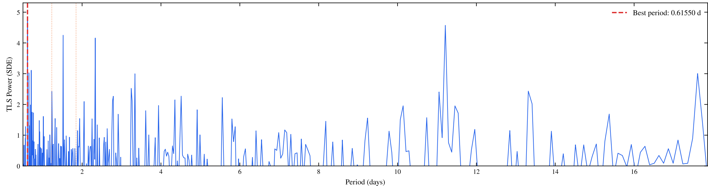
TIC 207081058 | Sectors: 105, 106 | TLS Coarse Periodogram (SDE = 4.82)
