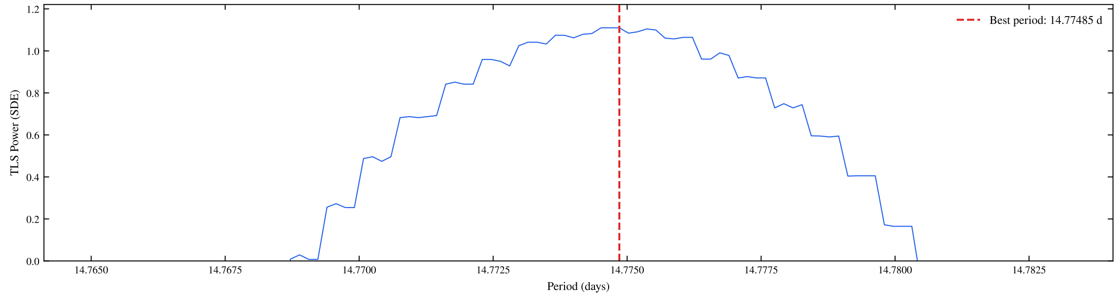
TIC 207081058 | Sectors: 105, 106 | TLS Coarse Periodogram (SDE = 1.11)
